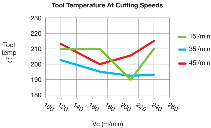
Figure 9: Temperature change at various cutting speeds
