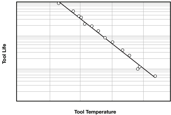
Figure 6: Typical tool life vs. temperature
