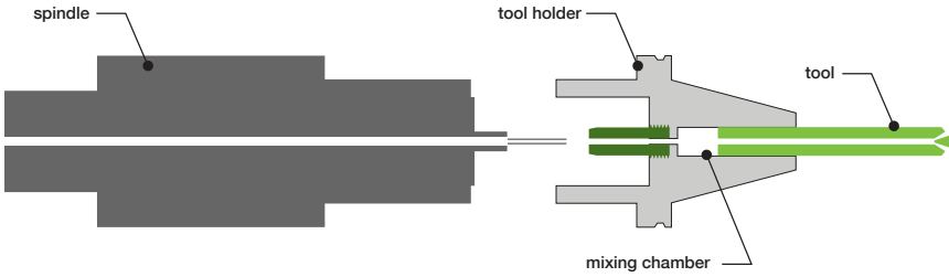
Figure 17: Dual-channel system components
