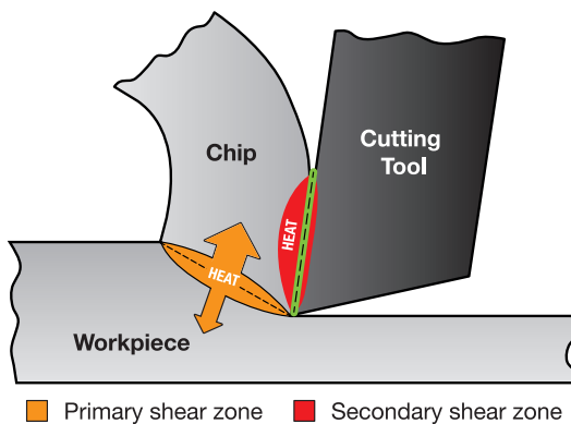
Figure 5: Heat generation in metal cutting
