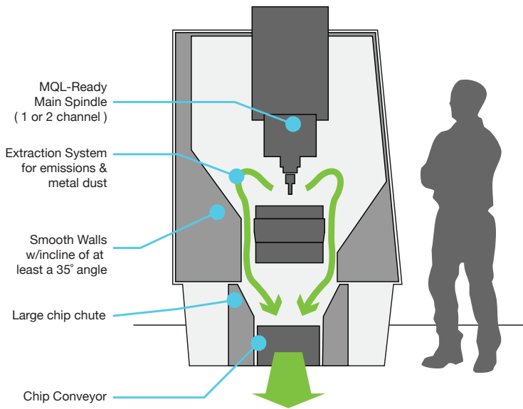
Figure 22: Elements of an MQL-specific machining center
