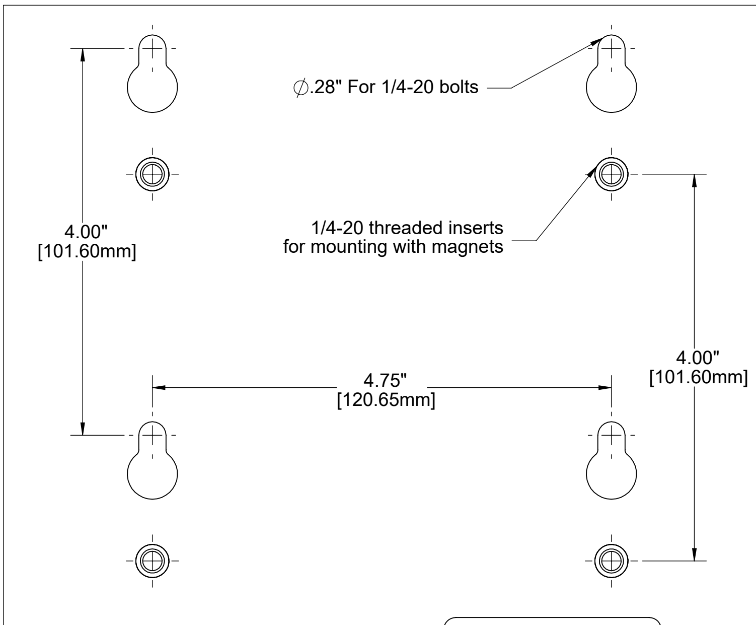
Drilling template for: 7.0" tall, enclosure weldment
